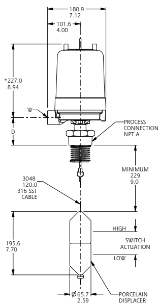
Drawing 0390670
