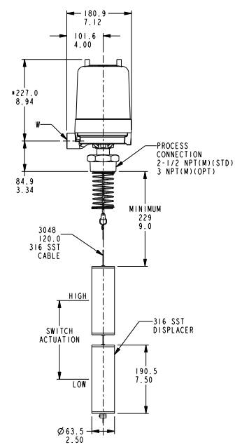
Drawing 0390673
