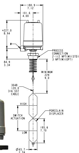
Drawing 0390672
