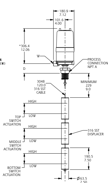
Drawing 0390682
