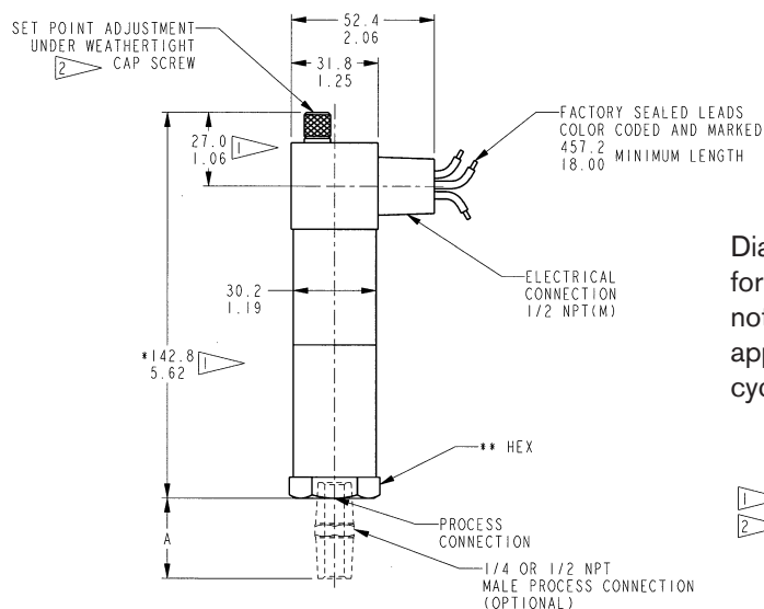
Drawing 0090179
