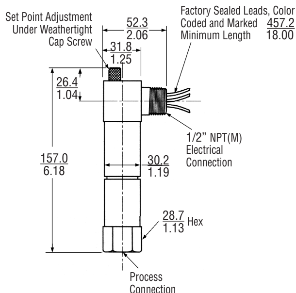
Drawing 0090179
