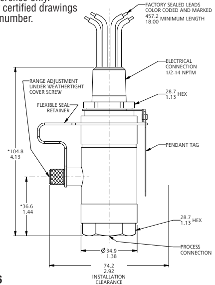
Drawing 0091356
