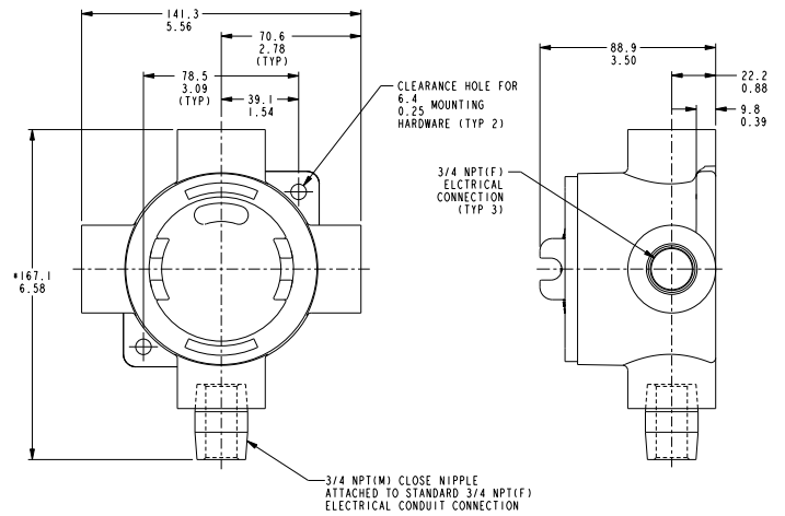
Drawing 0090300
