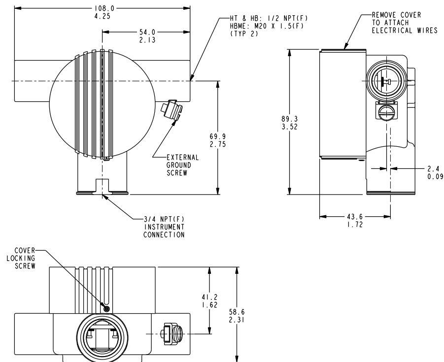
Drawing 0090763 Junction Box with Terminal Block: HT
